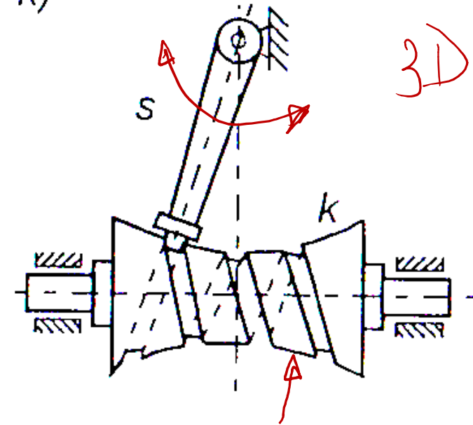
globoidal cam
