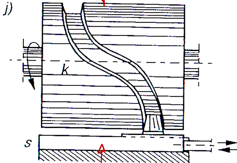
cylindrical cam
